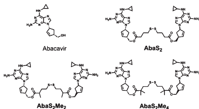
Figure 2. Structures of abacavir and abacavir prodrug homodimers: \text{AbaS}_2 , \text{AbaS}_2\text{Me}_2 , and \text{AbaS}_2\text{Me}_4 .
